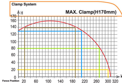
JIH-18C (D Type) Cutting Capacity Chart
