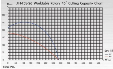
jih-t5s-26-1 45 degrees cutting capacity chart jih-t5s-26-1 90 degrees cutting capacity chart
